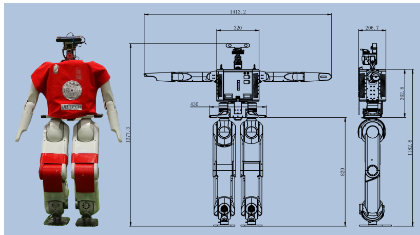
Fig. 1. Robot Walker
